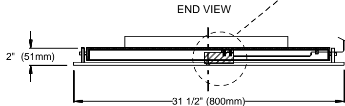
END VIEW
